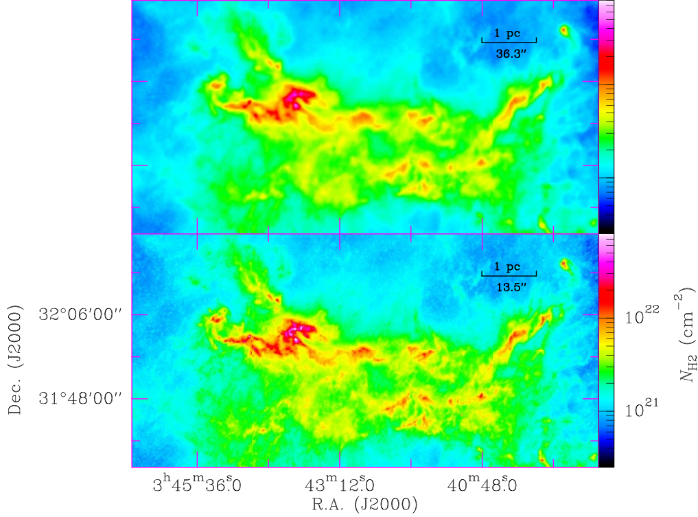
Figure 2. 13''.5 and 36''.3 resolution comparison. The top panel is a column density map with a resolution of 36''.3 . The bottom panel is a high-resolution column density image ( 13''.5 ) which is derived using an improved difference term algorithm. This algorithm uses all unresolved or slightly resolved structures for enhanced contrast.
