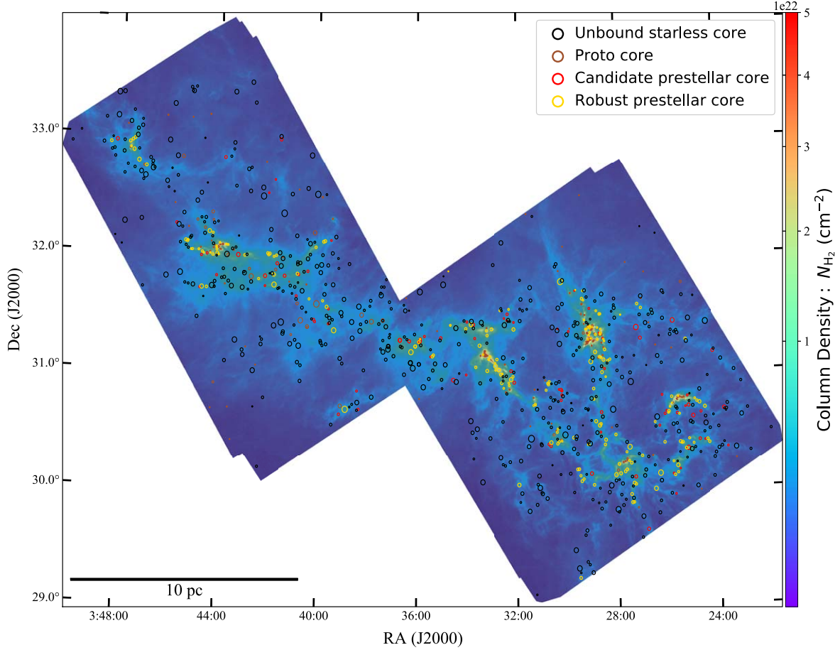
Figure 4. Positions of the 952 dense cores identified in the Perseus overlaid on the Herschel high resolution 13//5 column density map. Black, brown, red, and yellow circles mark the 536 unbound starless cores, the 130 protostellar cores, the 87 candidate prestellar cores, the 199 robust prestellar cores, respectively. The size of the circle is the geometric mean of the core's FWHM.
