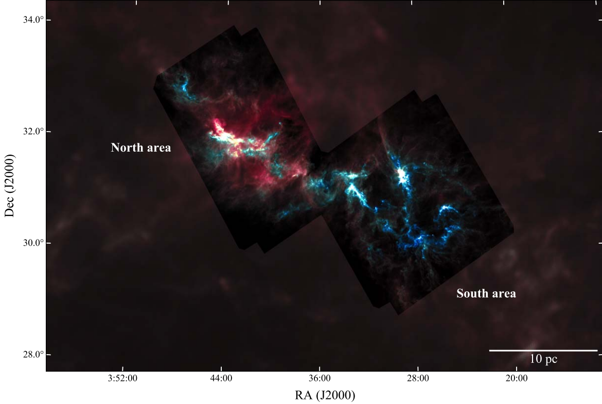
Figure 1. Red–Green–Blue (RGB) composites image showing the 250 \mu\text{m} (blue), 350 \mu\text{m} (green), and 500 \mu\text{m} (red) SPIRE fluxes for the Perseus molecular cloud derived from Herschel and Planck observations. In areas outside the Herschel coverage, dust models were applied to predict the corresponding SPIRE fluxes using Planck/IRAS data. Planck data have a lower resolution than Herschel’s, allowing us to identify their spatial boundaries.
