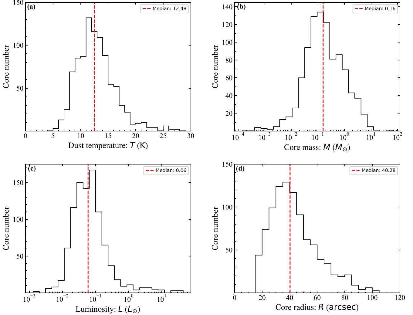
Figure 5. Histogram of physical parameters of the cores. Panels (a), (b), (c) show core dust temperature, mass and bolometric luminosity obtained from SED fitting. Panel (d) is the geometric mean of the core FWHMs. The red dashed lines mark the median value.
