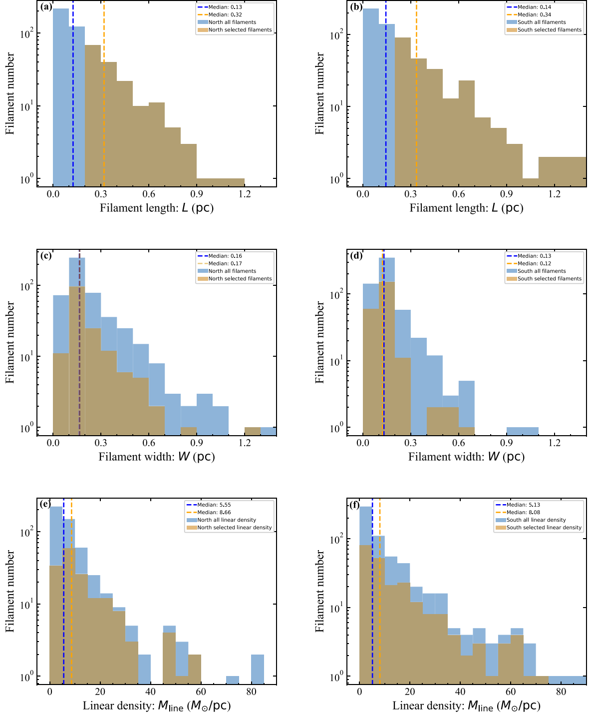
Figure 8. Histogram of physical parameters of the filamentary structures. In this set of histograms, the sample “all” are the filamentary structures with C > 0.5 ; the sample “selected” are the filamentary structures with C > 0.5 and L > 0.2 pc. We conduct separate statistics for filamentary structure in the north and south regions.
