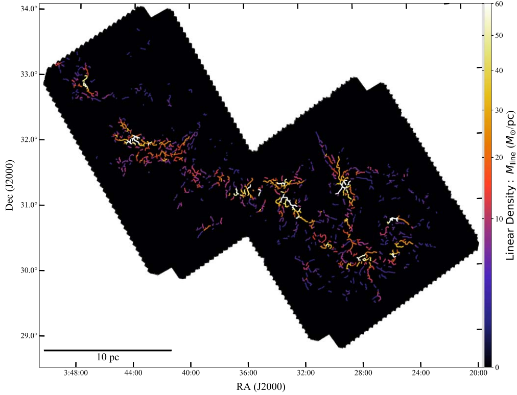
Figure 7. Perseus filamentary network structures selected with contrast C > 0.5 . The linear density ( M_{\text{line}} ) of the filamentary structure is only taken on the narrow side to avoid contamination as much as possible.
