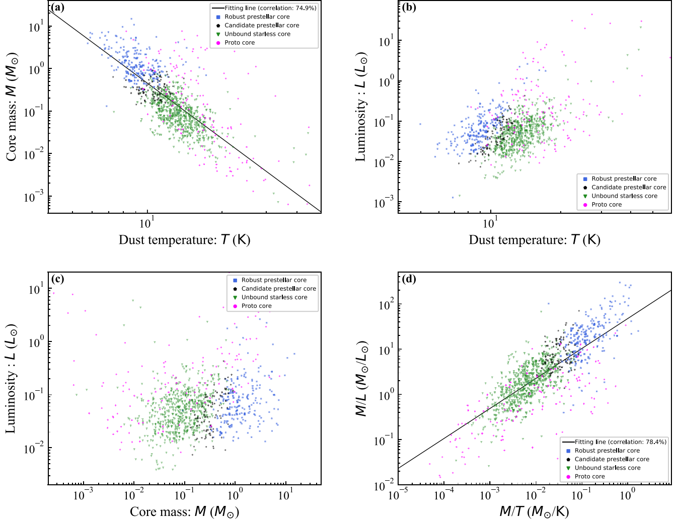
Figure 6. Correlations among core physical parameters derived by SED fitting. (a) A clear correlation between core dust temperature and mass, \log_{10}(M/M_{\odot}) = -4.34 \log_{10}(T/K) + 4 . (b), (c) Core luminosity has no significant correlation with dust temperature and mass. (d) A clear correlation between M/L and M/T , \log_{10}(M/T) = 0.66 \log_{10}(M/L) + 1.67 .
