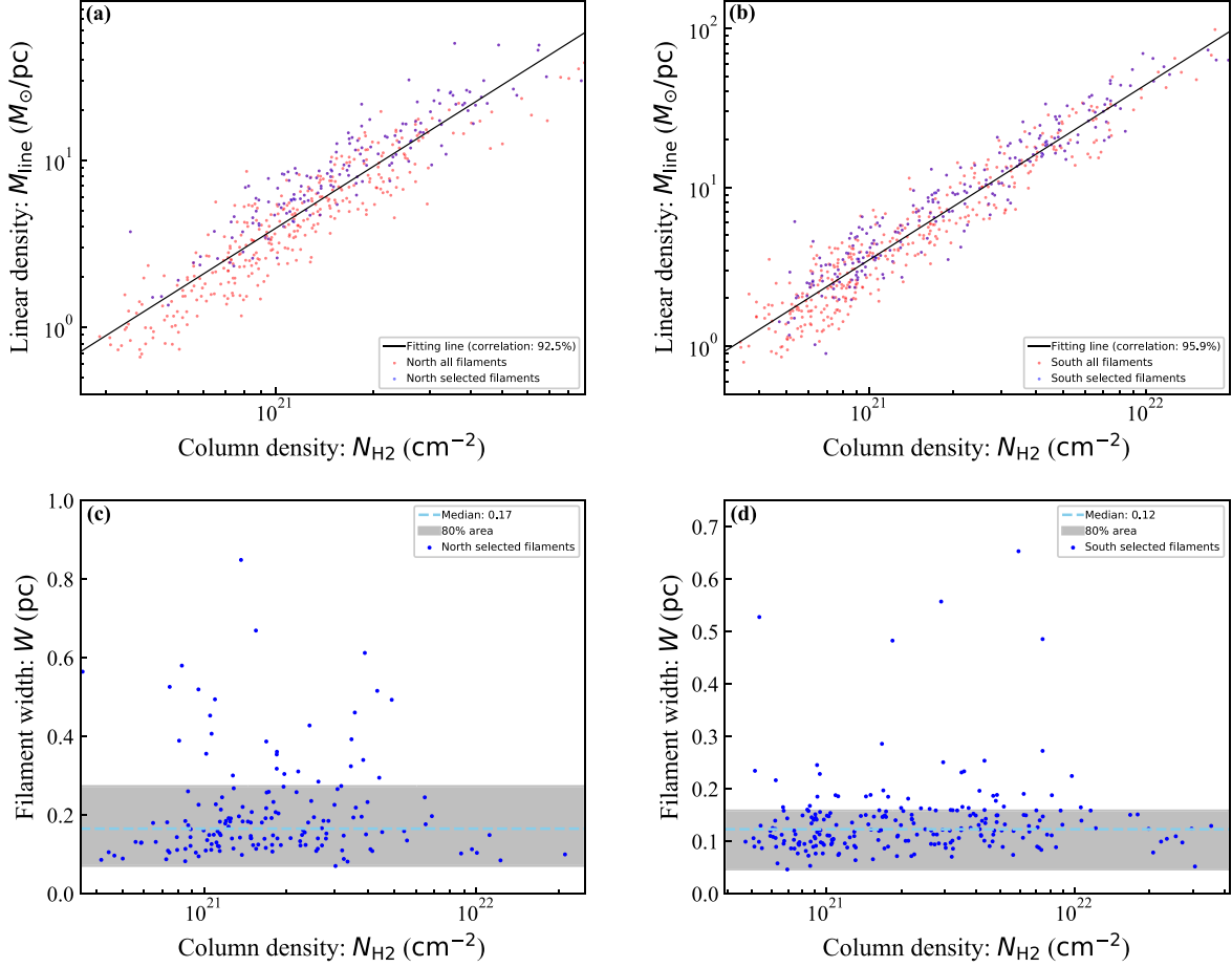
Figure 9. Crest column density ( N_{\text{H}_2} ) of filamentary structures as a function of linear density ( M_{\text{line}} ) and width ( W ) in the north and south regions of Perseus molecular cloud. N_{\text{H}_2} and M_{\text{line}} are clearly related. N_{\text{H}_2} are uncorrelated with W by three orders of magnitude from \sim 10^{20} to \sim 10^{22} \text{ cm}^{-2} .
