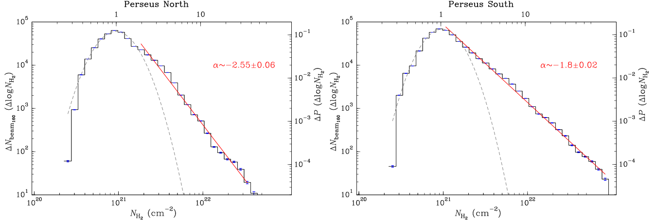
Figure 3. Probability distribution function (PDF) at 13''5 resolution of the column density map in Perseus north and south regions. The lower axis of the horizontal axis is the column density ( N_{\text{H}_2} ), the upper axis of the horizontal axis is the corresponding extinction A_V (mag).
