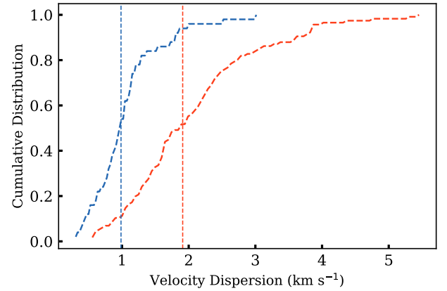
Figure 5. The velocity dispersion distributions for SiO clumps with outflows and without outflows (the red and blue lines). The vertical dashed lines represent the median velocity dispersion of SiO clumps in the two groups: 1.91 km s −1 (red line) and 0.99 km s −1 (blue line) for clumps with and without strong outflows, respectively.
