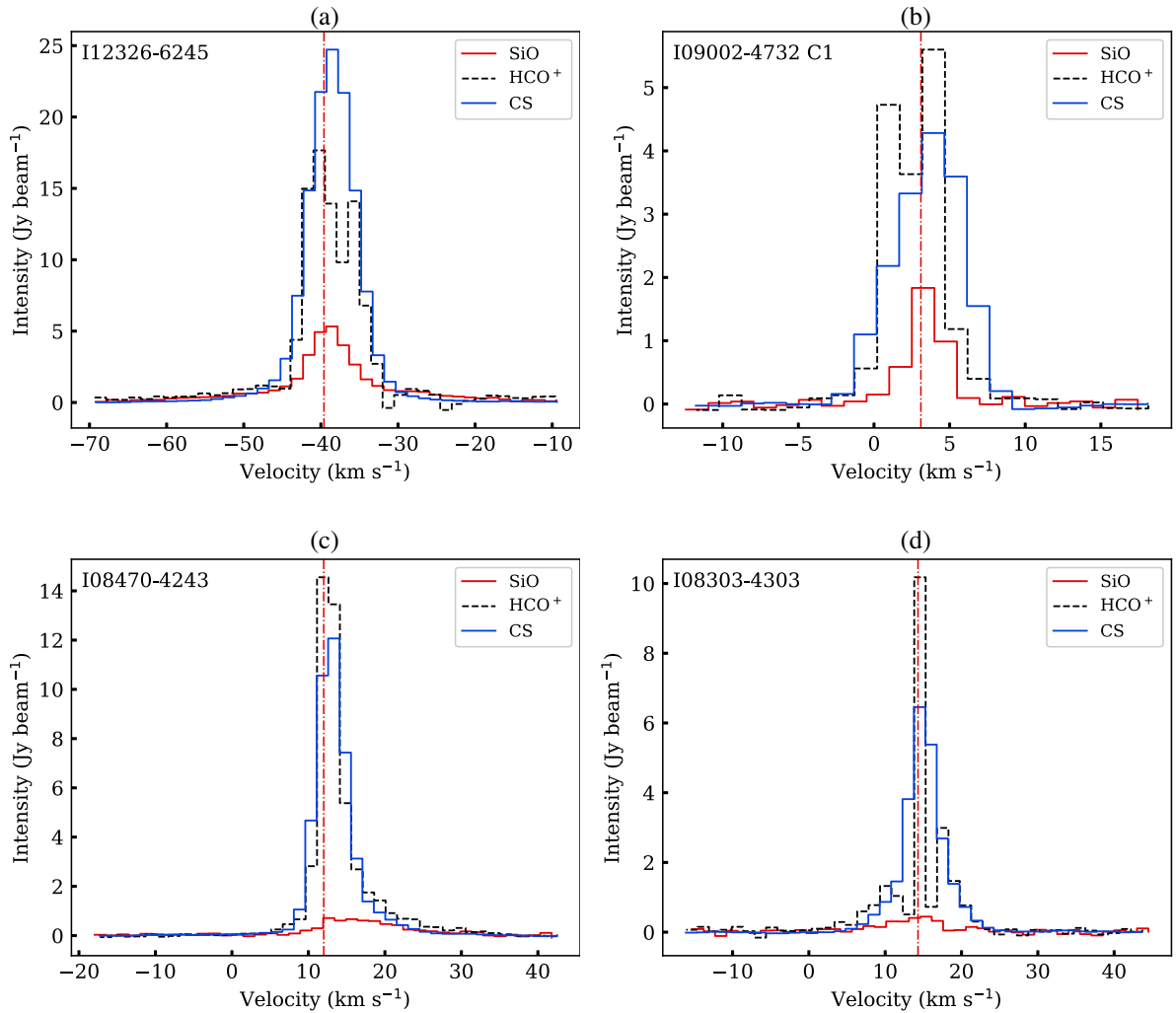
Figure 2. Examples of sources. The red spectrum represents the SiO average spectral extracted over the aperture of SiO clumps or beam. The \text{HCO}^+ and CS spectra are presented as black dashed and blue solid lines. The dash–dotted line indicates the systemic velocity of the source.
